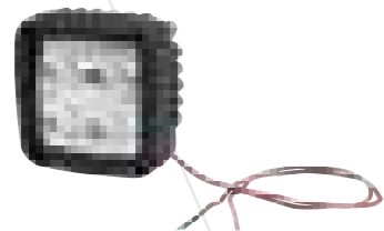
Work Lamp-Square LA10091 Lumen 3200 Dimensions 97 x 114 x 74mm
