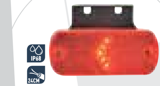
Rear Position Light-Red LA30108 LED Dimensions 105.4 x 45mm
