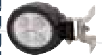
Work Lamp-Oval LA10018 Lumen 1500 Dimensions 120 x 104 x 81
